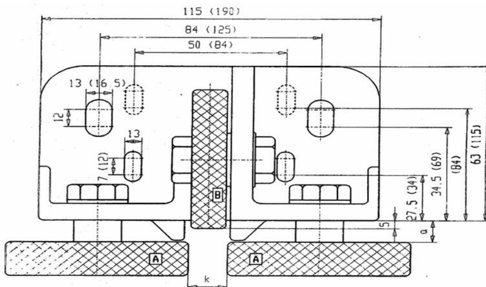
Dimensions GG (differing dimensions for FK in parenthesis)
